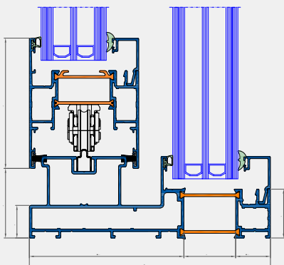
Verticale doorsnede (monorail)
